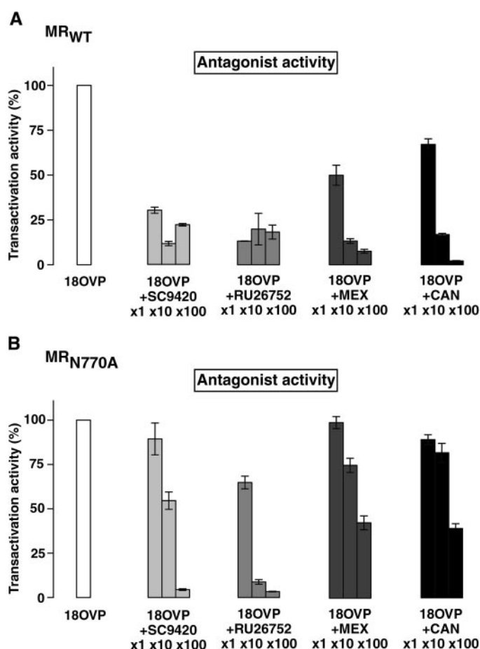
Fig. 9. Transactivation properties of MR WT and MR N770A in response to spirolactones. HEK 293T cells transiently expressing MR WT (A) or MR N770A (B) were incubated for 24 h with 10 -7 M 18OVP in the absence (100% agonist activity) or presence of increasing (10 -7 M–10 -5 M) concentrations of the spirolactones tested. Transactivation activities of MRs were determined from the luciferase activity normalized in terms of the \beta -galactosidase activity. Values are mean \pm S.E.M. of three separate experiments.
