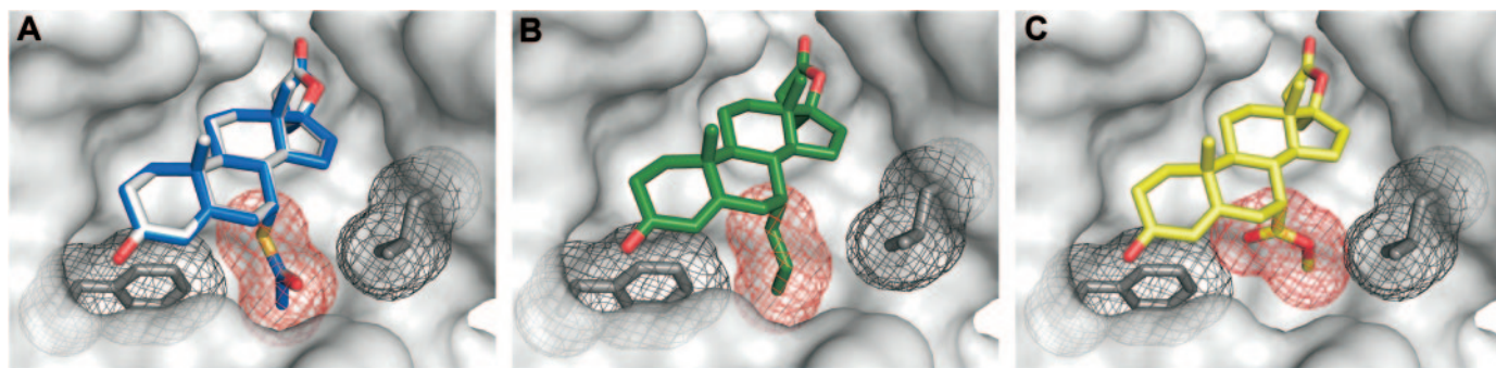
Fig. 6. Spirolactones within the ligand-binding cavity of MR_{S810L} . A, superimposition of the minimized SC9420 (blue) over the SC9420 in the crystal structure (gray) within the ligand-binding cavity of MR_{S810L} . Docking of the lowest energy conformations of RU26752 (B) and mexrenone (C) within the ligand-binding cavity of MR_{S810L} . Van der Waals volumes of the C7 substituent are depicted in red and those of Phe829 and Leu938 in black. The figure was generated using Open PyMol version 0.93.
