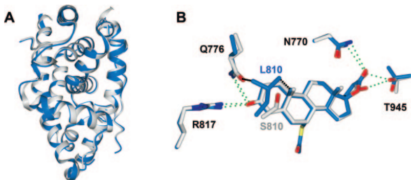
Fig. 5. Superimposition of the structure of the LBD of MR S810L associated with SC9420 (blue) over that of MR WT , associated with deoxycorticosterone (gray) (PDB ID 2ABI). A, overall organization of the LBDs. B, focus on the ligand-binding cavities. Hydrogen bonds and van der Waals interactions are depicted as dashed green and black lines, respectively. This figure was produced using DINO ( http://www.dino3d.org ).
