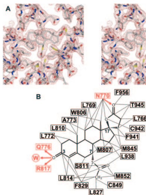
Fig. 3. Crystal structure of the MR S810L -LBD associated with SC9420. A, stereo view of the 2F_o - F_c electron density map showing SC9420, and the surrounding residues in the MR S810L -LBD. The map was calculated at 2.29 Å and contoured at 1 \sigma . This figure was produced using DINO ( http://www.dino3d.org ). B, diagram showing the interactions between MR S810L -LBD and SC9420. Hydrogen bonds and van der Waals interactions are depicted as solid red arrows and dashed black lines, respectively. W indicates a water molecule.
