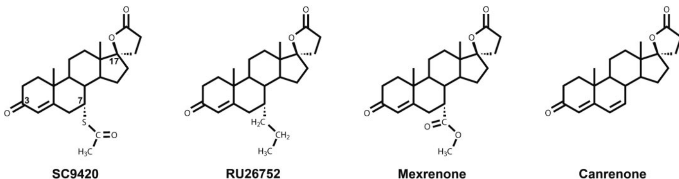
Fig. 1. Structural formulae of spirolactones.
