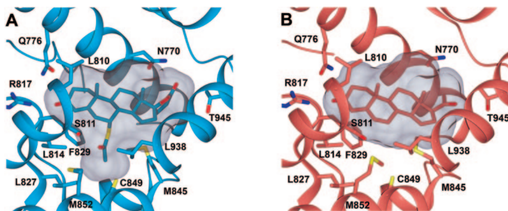
Fig. 4. Ligand-binding pockets of MR S810L -LBD associated with SC9420 (A) and progesterone (PDB ID 1YA3) (B). The ligand cavities volumes (gray) were calculated by VOIDOO (Kleywegt and Jones, 1994). This figure was produced using DINO ( http://www.dino3d.org ).
