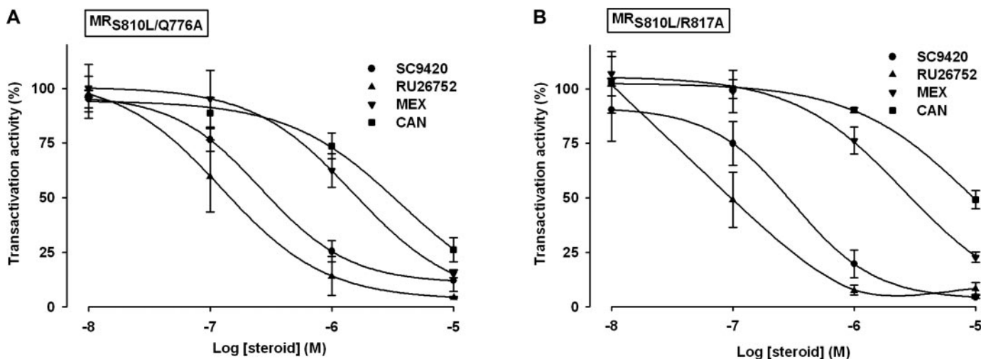
Fig. 7. Transactivation properties of MR_{S810L/Q776A} and MR_{S810L/R817A} in response to spirolactones. HEK 293T cells transiently expressing MR_{S810L/Q776A} (A) and MR_{S810L/R817A} (B) were incubated for 24 h with 10^{-7} M aldosterone in the absence (100% agonist activity) or presence of increasing ( 10^{-8} M to 10^{-5} M) concentrations of SC9420, RU26752, mexrenone (MEX), and canrenone (CAN). Transactivation activities of mutant MRs were determined from the luciferase activity normalized in terms of the \beta -galactosidase activity. Values are mean \pm S.E.M. of three separate experiments.
